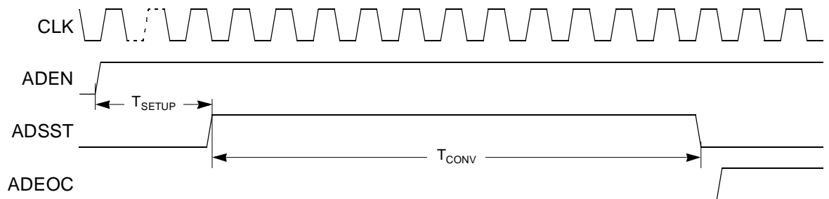
Figure 47. Timing Diagram
