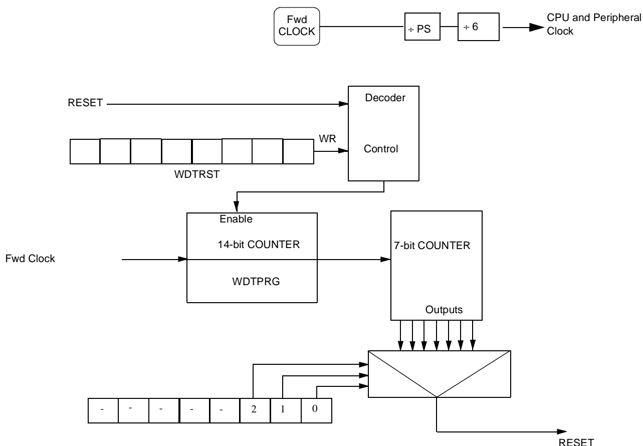
Figure 29. WatchDog Timer
