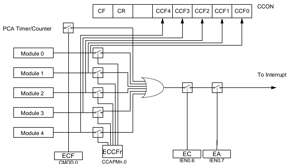
Figure 41. PCA Interrupt System
