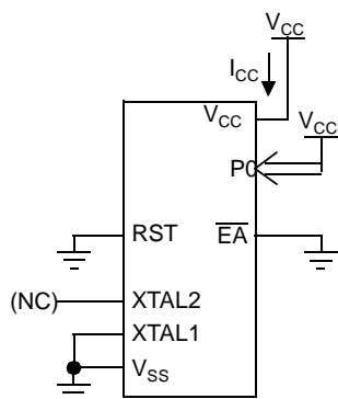
Figure 60. I_{CC} Test Condition, Power-Down Mode
