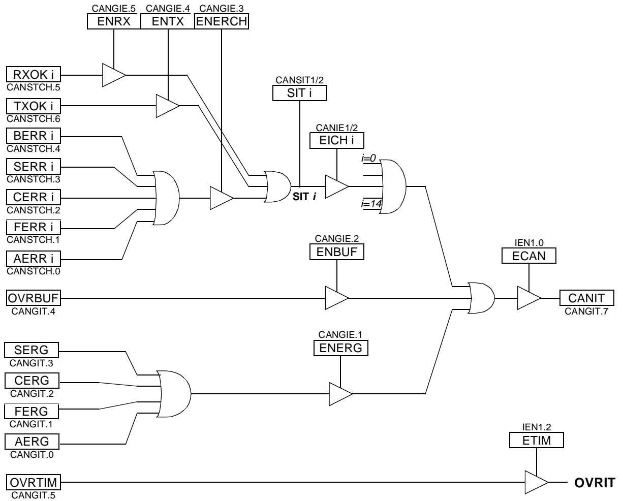
Figure 33. CAN Controller interrupt structure
