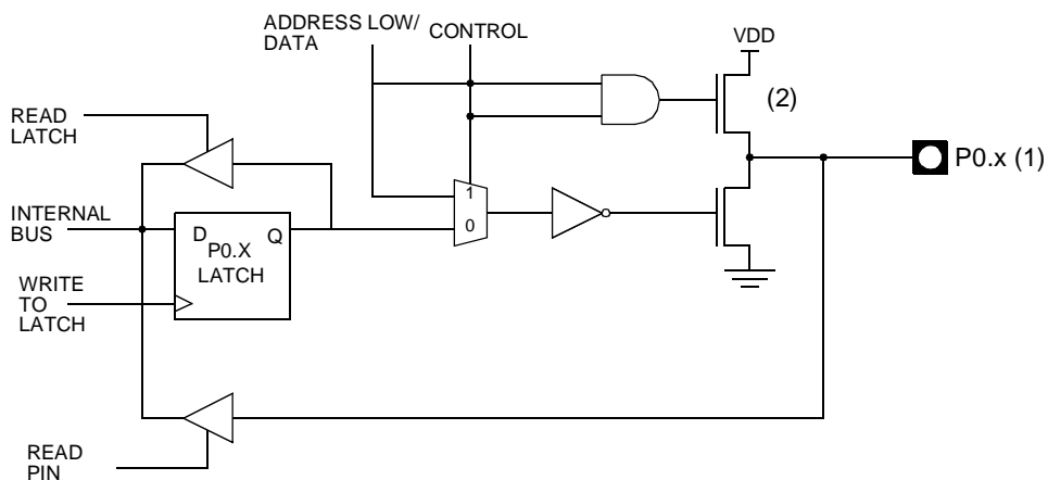
Figure 2. Port 0 Structure
