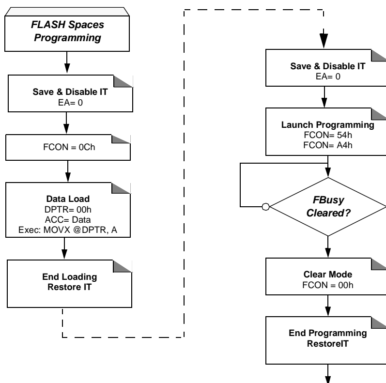
Figure 14. Hardware Programming Procedure
