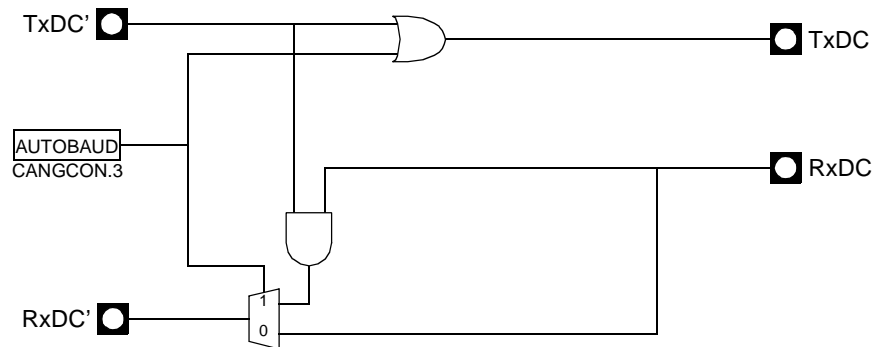
Figure 39. Autobaud Mode
