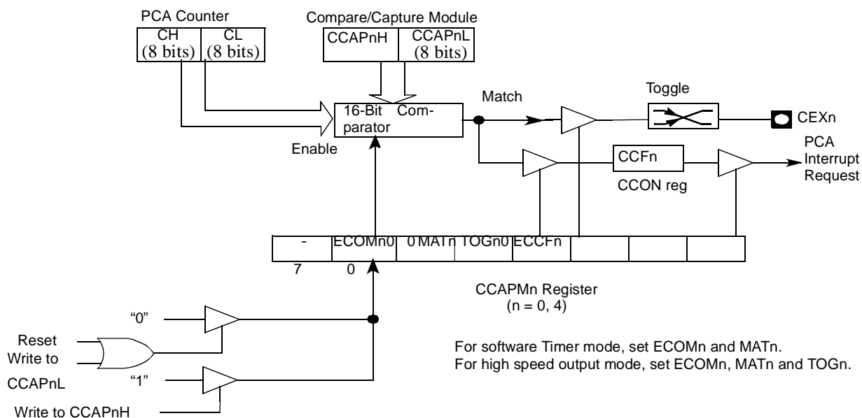
Figure 43. PCA 16-bit Software Timer and High Speed Output Mode
