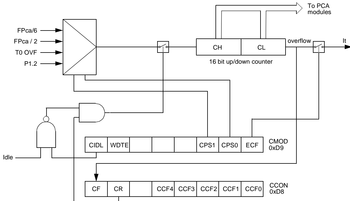
Figure 40. PCA Timer/Counter
