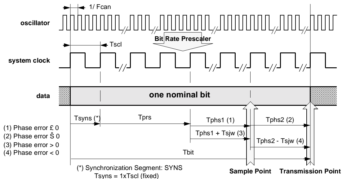
Figure 35. General structure of a bit period
