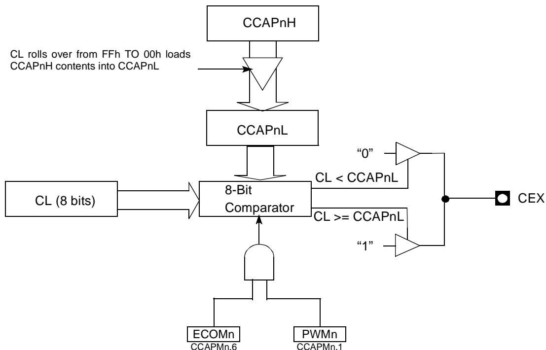
Figure 45. PCA PWM Mode
