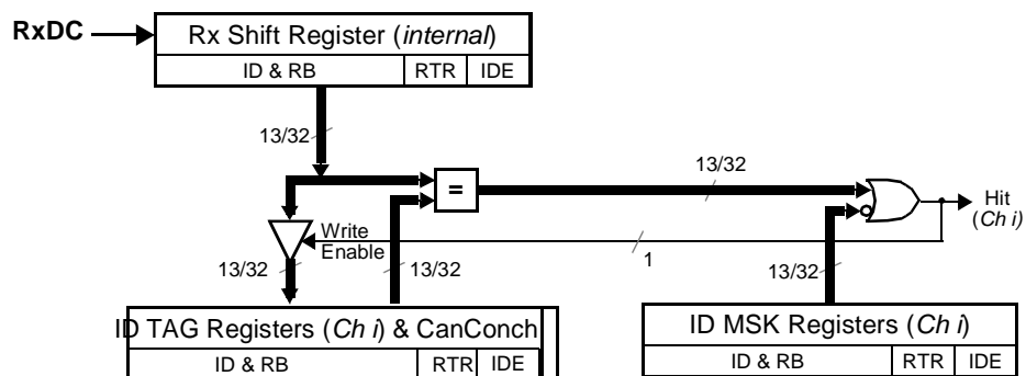
Figure 37. Acceptance filter block diagram
