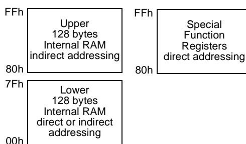
Figure 1. Internal memory - RAM
