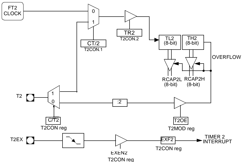
Figure 28. Clock-Out Mode
