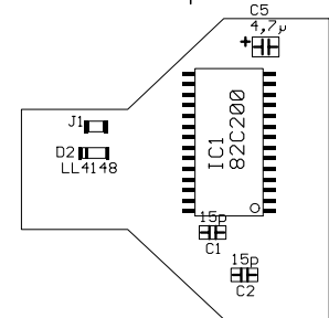
CAN-Adapter (Vers. 2)
